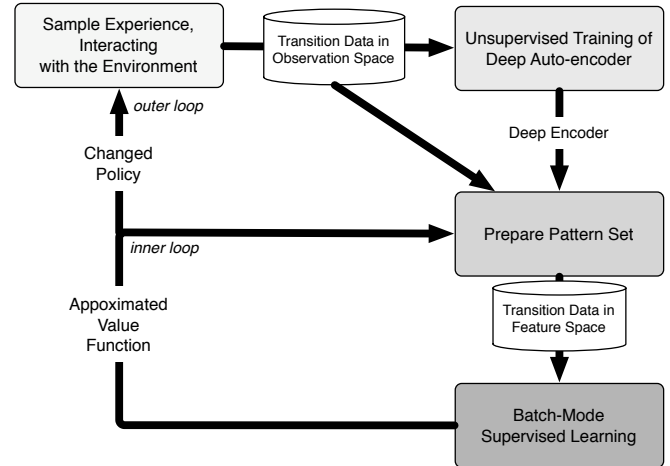
Fig. 3. Graphical sketch of the proposed framework for deep batch-RL with episodic exploration.
